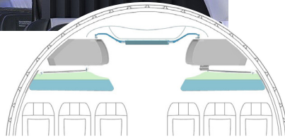
B737 PSU mounted Class Divider for staggered installation
